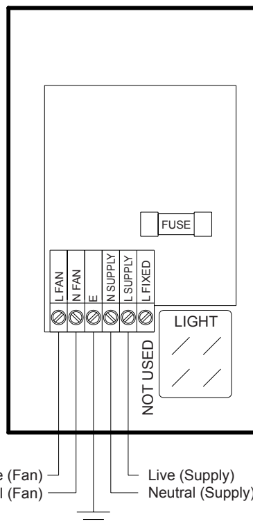
V65E & V20E Wiring diagram - internal view
