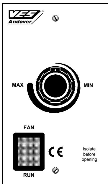
V65E & V20E External view of front panel
